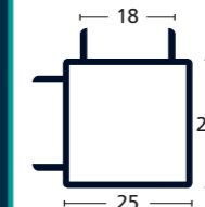
SAPPHIRE PROFRAME ALUMINIUM DOUBLE FIN ON 2 FACES SQUARE TUBE 25 x 25mm
