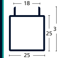
SAPPHIRE PROFRAME ALUMINIUM DOUBLE FIN ON 1 FACE SQUARE TUBE 25 x 25mm
