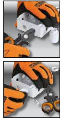
Profile and mill: designed to enlarge holes on plastic, from 13 mm to 24 mm.
